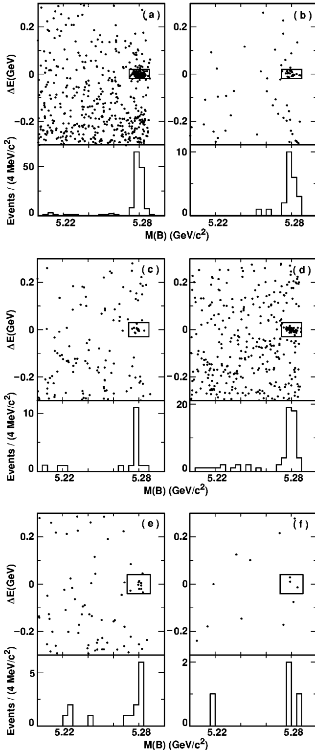
FIG. 1. \Delta E vs M(B) for (a) B^+ \rightarrow \psi(2S)K^+ , (b) B^0 \rightarrow \psi(2S)K_S^0 , (c) B^+ \rightarrow \psi(2S)K^{*+} , K^{*+} \rightarrow K_S^0 \pi^+ , (d) B^0 \rightarrow \psi(2S)K^{*0} , K^{*0} \rightarrow K^+ \pi^- , (e) B^+ \rightarrow \psi(2S)K^{*+} , K^{*+} \rightarrow K^+ \pi^0 , and (f) B^0 \rightarrow \psi(2S)K^{*0} , K^{*0} \rightarrow K_S^0 \pi^0 candidate events, with the contributions from \psi(2S) \rightarrow l^+ l^- and \psi(2S) \rightarrow J/\psi \pi^+ \pi^- combined. The boxes indicate the signal regions. Also shown are the M(B) projections for the candidate events with \Delta E within the signal area limits.
